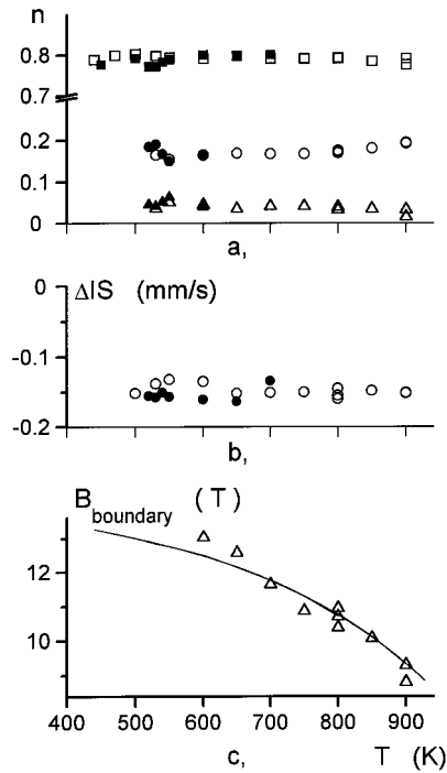
Figure 3. Temperature dependence of the Mössbauer parameters of ncFe_{90}Zr_7B_2Cu_1 in the as-formed nanocrystalline state (empty symbols) and after the 900 K annealing (full symbols). The relative amount of Fe atoms in the nanocrystalline bcc phase (squares), in the residual amorphous phase (circles), in the boundary region (empty triangle) and after its crystallization (full triangles) are shown in (a). \Delta IS = IS_m - IS_{am} , the difference between the isomer shifts of the main nanocrystalline line ( IS_m ) and the residual amorphous phase ( IS_{am} ), is shown in (b). The temperature dependence of the hyperfine field of the boundary region, B_{boundary} is shown to follow that of the main nanocrystalline component B_m (continuous line) in (c). The results of three independent measurements at 800 K show the typical statistical and systematical errors of the evaluation.
