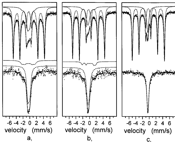
Figure 1. Mössbauer spectra of ncFe_{84}Zr_7B_6Cu_1 and ncFe_{90}Zr_7B_2Cu_1 taken above T_c^a at T = 650 K in the as-formed nanocrystalline state (a and b, respectively) and for ncFe_{90}Zr_7B_2Cu_1 after the 900 K annealing (c). The full lines are the fitted curves, their nanocrystalline component and their residual part are marked with the broken and dotted lines, respectively. In the lower half of the figure the residual spectra obtained after the subtraction of the nanocrystalline components are shown and in the as received states the components attributed to the residual amorphous phase (broken line) and to the boundary region (dotted line) are also shown.
