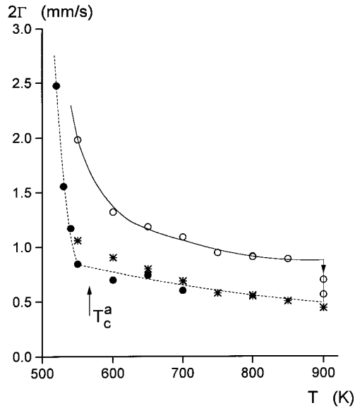
Figure 4. Temperature dependence of the linewidth of the residual amorphous phase in the as-formed state (open circles) and after the 900 K annealing (full circles). The stars correspond to the linewidth in the as-formed state obtained after the removal of the broadening due to the inner field of the magnetic domains, see text. The continuous and dotted lines are guides to the eye.
