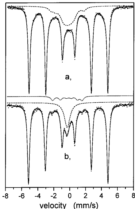
Figure 2. Mössbauer spectra of ncFe_{90}Zr_7B_2Cu_1 taken below T_c^a at T = 550 K in the as-formed nanocrystalline state (a) and after the 900 K annealing (b). The full lines are the fitted curves, in (a) the residual part beside the nanocrystalline components is marked with a broken line; in (b) the components attributed to the residual amorphous phase (broken line) and to the crystallized boundary region (dotted line) are shown.
